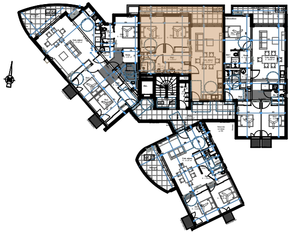
PLAN R+1
