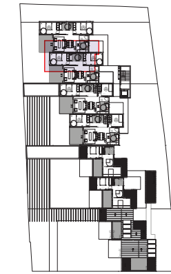
PLAN R+5
